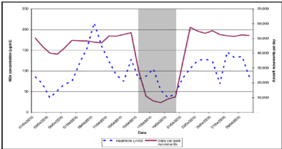
UK airspace closure April 2010 - daily average NOx concentrations measured at Heathrow Airport compared to total daily car park movements
