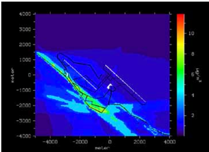
NOx dispersion during airspace closure with remaining handling and airport sources and reduced landside vehicle traffic [17.4.2010]
