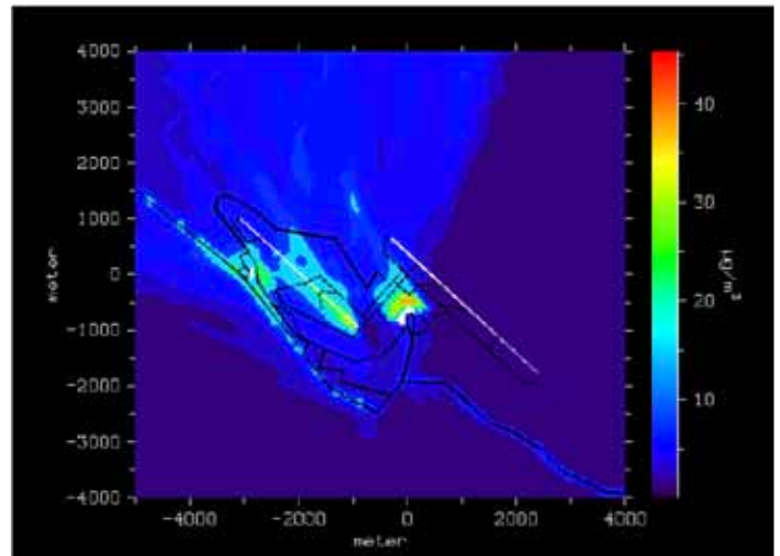
NOx dispersion of all airport related sources (aircraft (performed based), handling, other airport sources, landside car traffic) [24.4.2010]
