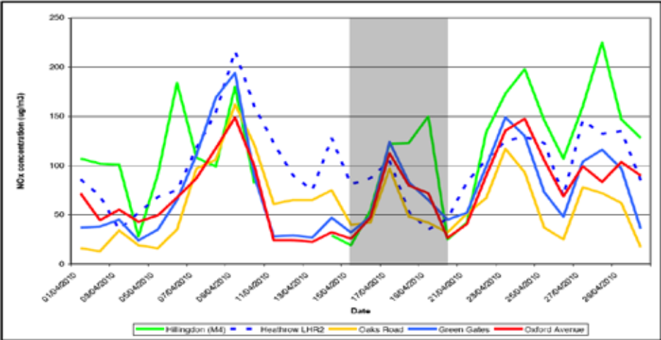
UK airspace closure April 2010 - daily average NOx concentrations measured at selected sites on and around Heathrow
