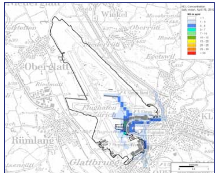
NO 2 dispersion during airspace closure with remaining handling and airport sources and reduced landside car traffic [18.4.2010]
