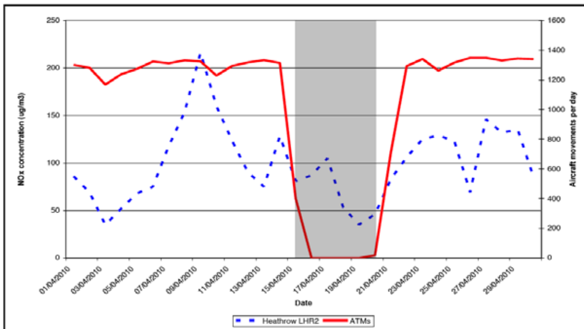
UK airspace closure April 2010 - daily average NOx concentrations measured at Heathrow Airport compared to daily aircraft movements
