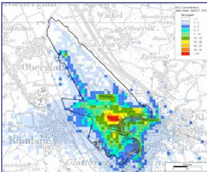
NO 2 dispersion of all airport related sources (aircraft (performed based), handling, other airport sources, landside car traffic) [27.4.2010]
